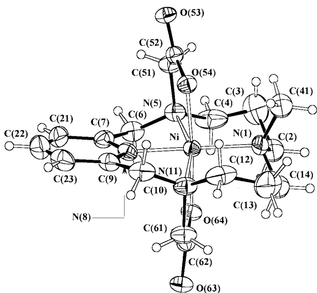
Fig. 2 The molecular structure of [\text{Ni}(\text{HL}^1)]^+ 2^+ with the labelling scheme adopted.
